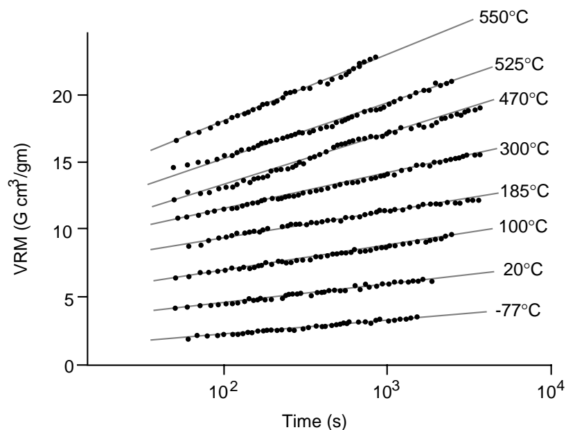
Figure 3.19 Progressive acquisition of VRM by synthetic sample of dispersed 2- \mu\text{m} diameter grains of magnetite. Data points show VRM acquired at corresponding time since the beginning of exposure to the magnetic field; lines show the trend of VRM for a particular VRM acquisition experiment at the temperature indicated; the magnetic field was 3.3 Oe; zero on the ordinate is arbitrary (the absolute value of VRM was adjusted so that results of all VRM acquisition experiments could be conveniently shown on a single drawing). Redrawn from Stacey and Banerjee (1974).
