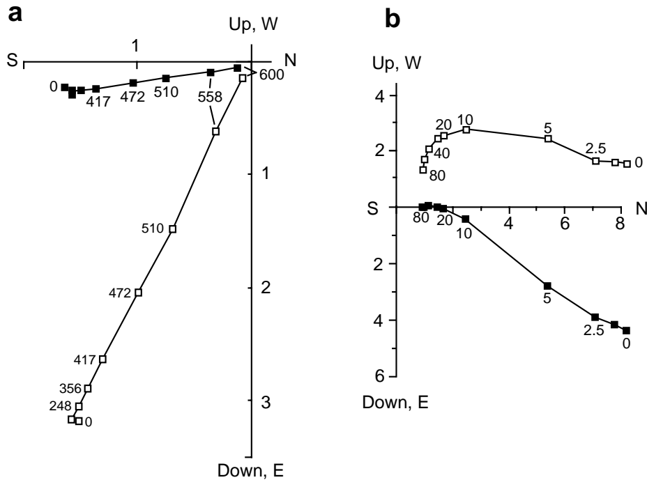
Figure 5.18 Vector component diagrams. (a) Progressive thermal demagnetization results for one sample; the numbers adjacent to data points are temperatures in degrees Celsius; open data points are vector end points projected onto a north-south oriented vertical plane; solid data points are vector end points projected onto the horizontal plane; numbers on axes are in A/m. (b) Progressive AF demagnetization results for another sample. Conventions and labels as for part (a) , except that numbers adjacent to the data points indicate H_{AF} (in mT); the NRM of this sample contains a large secondary lightning-induced IRM.
