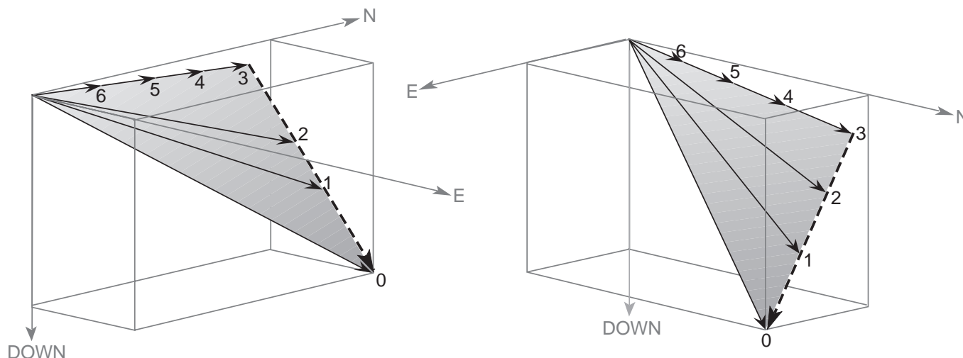
Figure 5.3 Perspective diagram of NRM vector during progressive demagnetization. Geographic axes are shown; solid arrows show the NRM vector during demagnetization at levels 0 through 6; the dashed arrow is the low-stability NRM component removed during demagnetization at levels 1 through 3; during demagnetization at levels 4 through 6, the high-stability NRM component decreases in intensity but does not change in direction.
