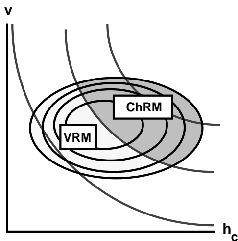
Figure 5.17 Grain volume ( v ) versus microscopic coercive force ( h_c ) for a hypothetical population of SD grains. Symbols and contours as in Figure 5.2.
