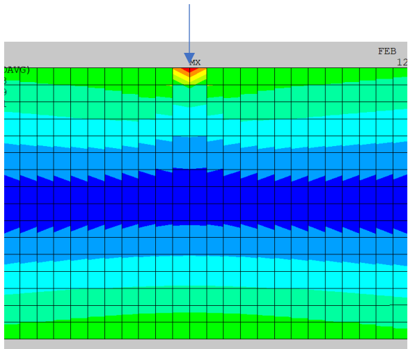
FEA Results showing point load at the top of a beam.
