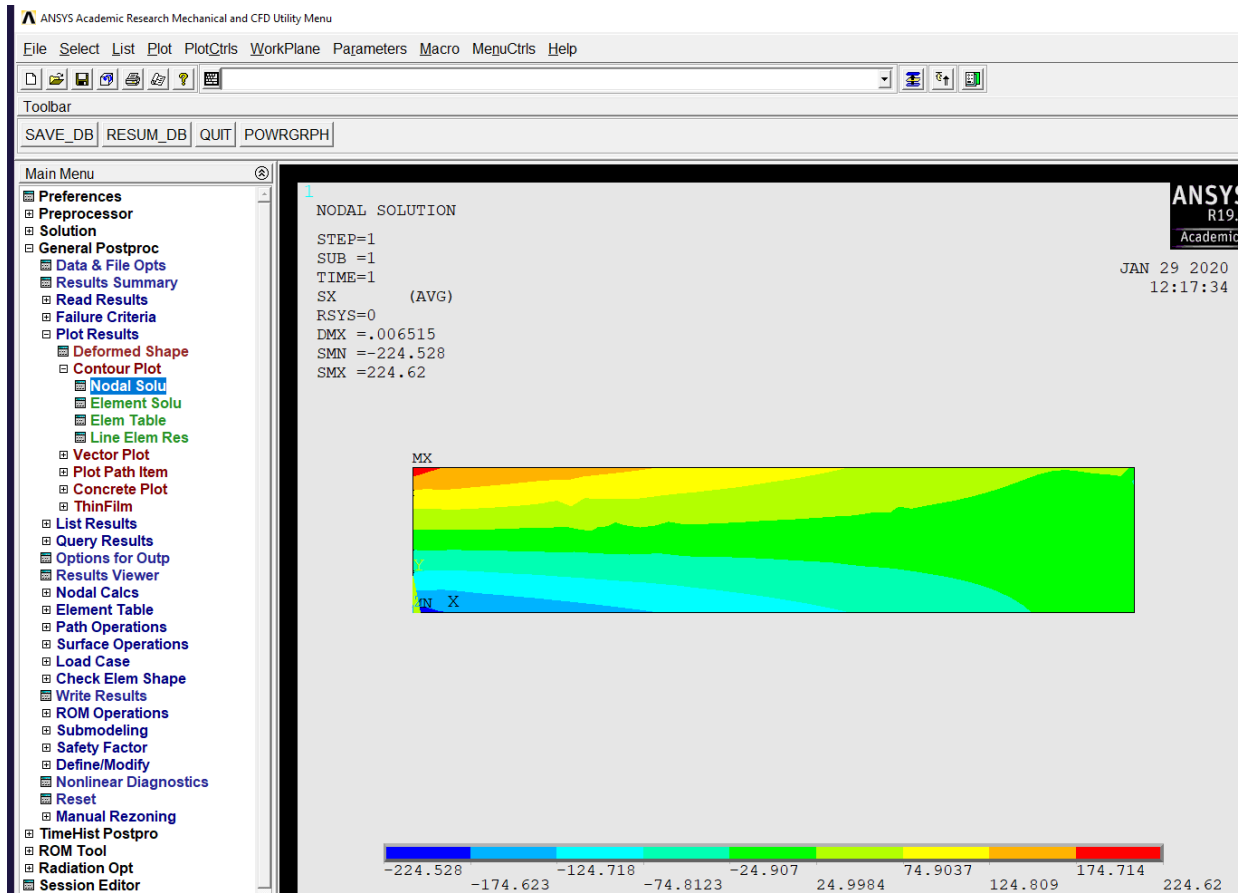
FEA output (x-direction stress), hw2, prob 4, PLANE182 elements. 5kN load applied at end
