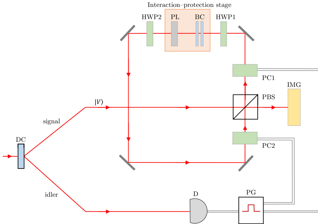
FIG. 1. Proposed scheme for a photonic implementation of a protective measurement based on the quantum Zeno effect. A vertically polarized signal photon resulting from a down-conversion process (DC) is reflected into the optical loop at the polarizing beam splitter (PBS). Upon leaving the PBS, brief activation of a Pockels cell (PC1) by a pulse generator (PG), which is triggered by the arrival of the idler photon at a detector (D), changes the polarization of the signal photon to horizontal. The signal photon then traverses an interaction-protection stage consisting of two half-wave plates (HWPs), a pair of birefringent crystals (BCs), and a linear polarizer (PL). HWP1 prepares the initial quantum state |\psi\rangle = \cos\theta|H\rangle + \sin\theta|V\rangle . BC implements a small polarization-dependent spatial displacement of the photon, weakly coupling polarization and spatial degrees of freedom. PL realizes the state protection by projecting the photon back onto the initial state |\psi\rangle . HWP2 rotates the polarization to horizontal, thereby readying the photon for transmission at the PBS for its next round trip through the loop. After N such round trips, a second Pockels cell (PC2) is activated to rotate the polarization to vertical and switch the photon out of the loop to be detected at the spatially resolving photon imager (IMG).
